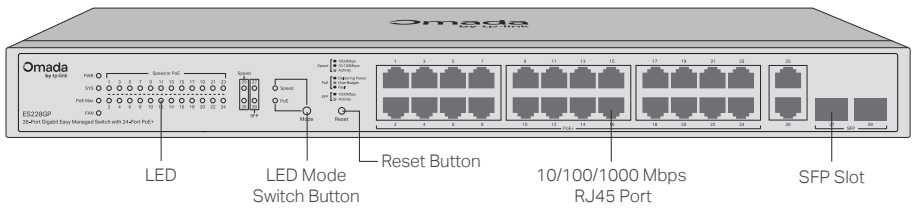
Figure 1-6 Front Panel of ES228GP
