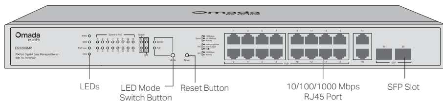
Figure 1-3 Front Panel of ES220GMP
