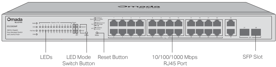
Figure 1-5 Front Panel of ES228GMP
