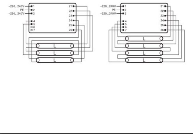
Wiring diagram
