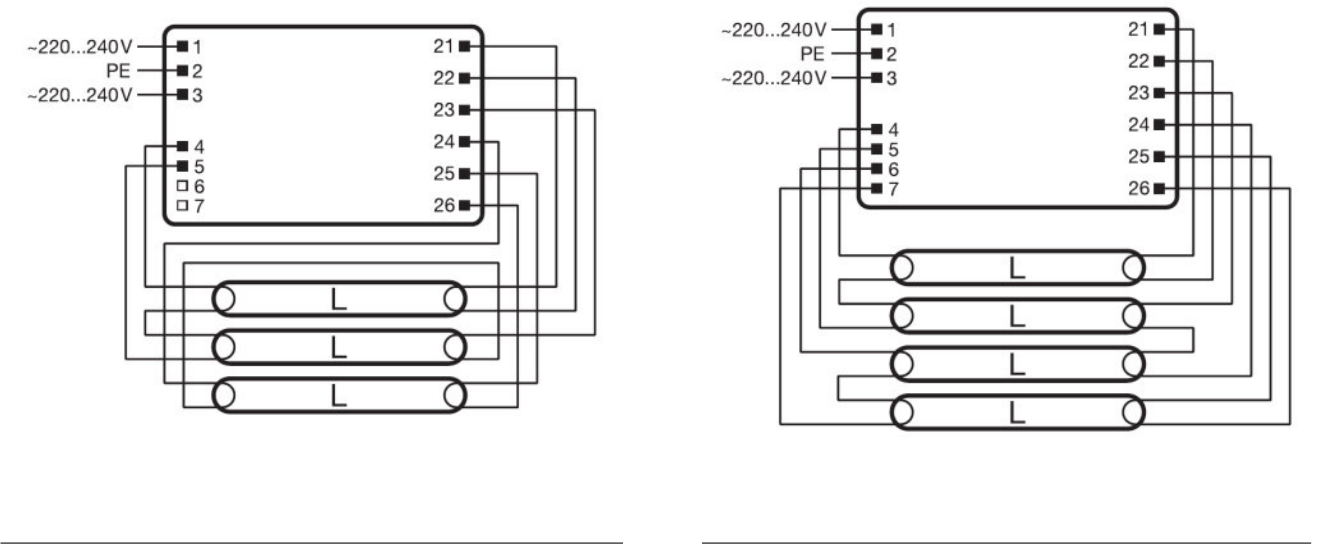
Wiring diagram
