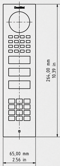
Front panel
