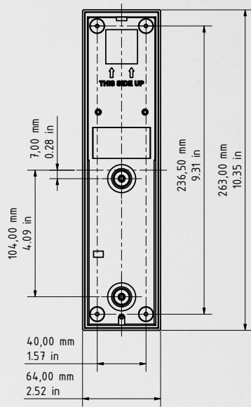
Surface-mounting housing (backbox)
