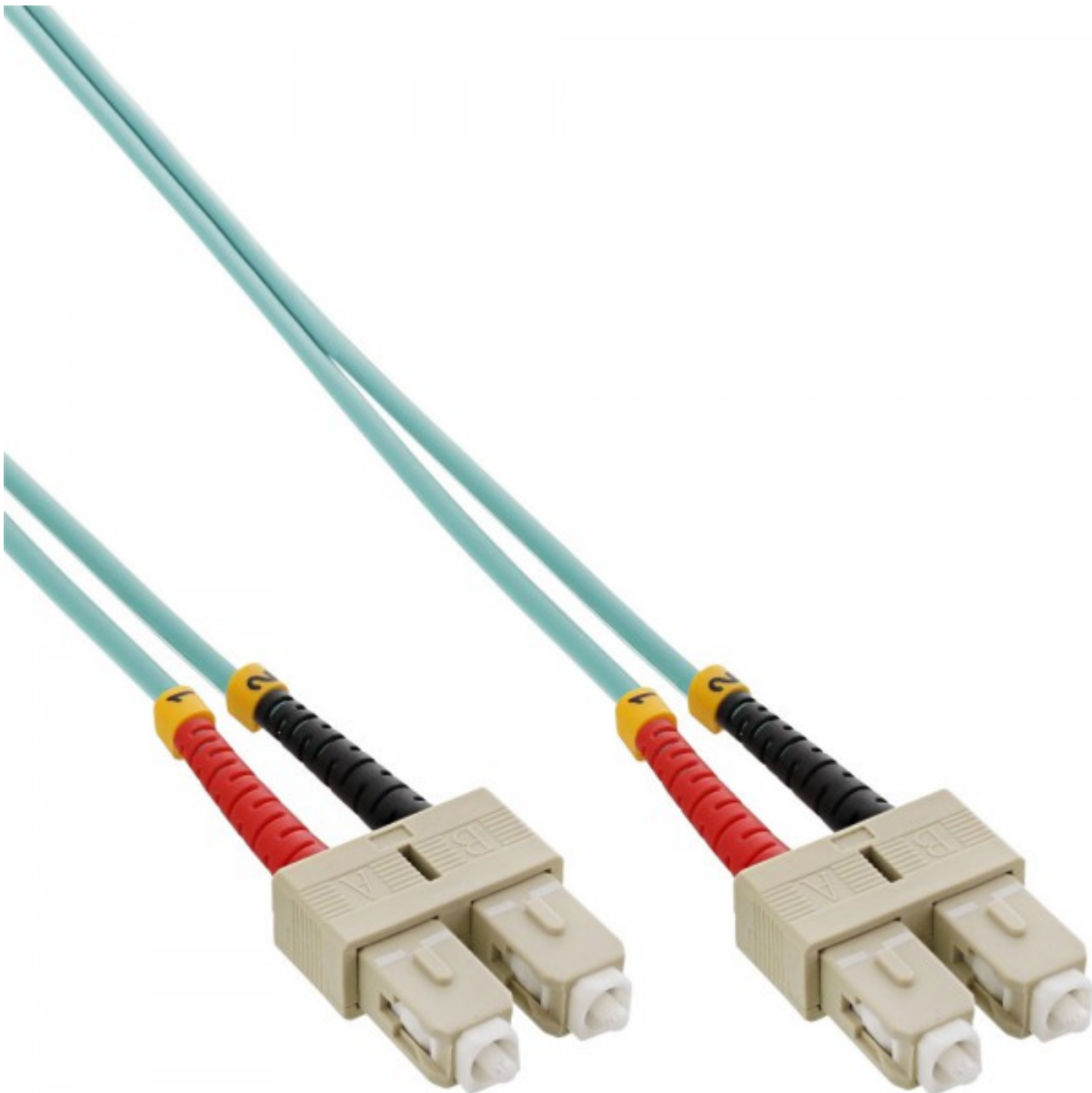
InLine® Fiber Optical Duplex Cable SC/SC 50/125µm OM3 7.5m
